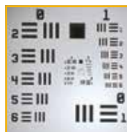
OGRASCOPTIC (22.63 LP/mm)
